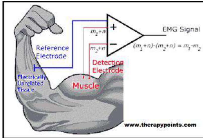
Figure 7: EMG Acquisition
