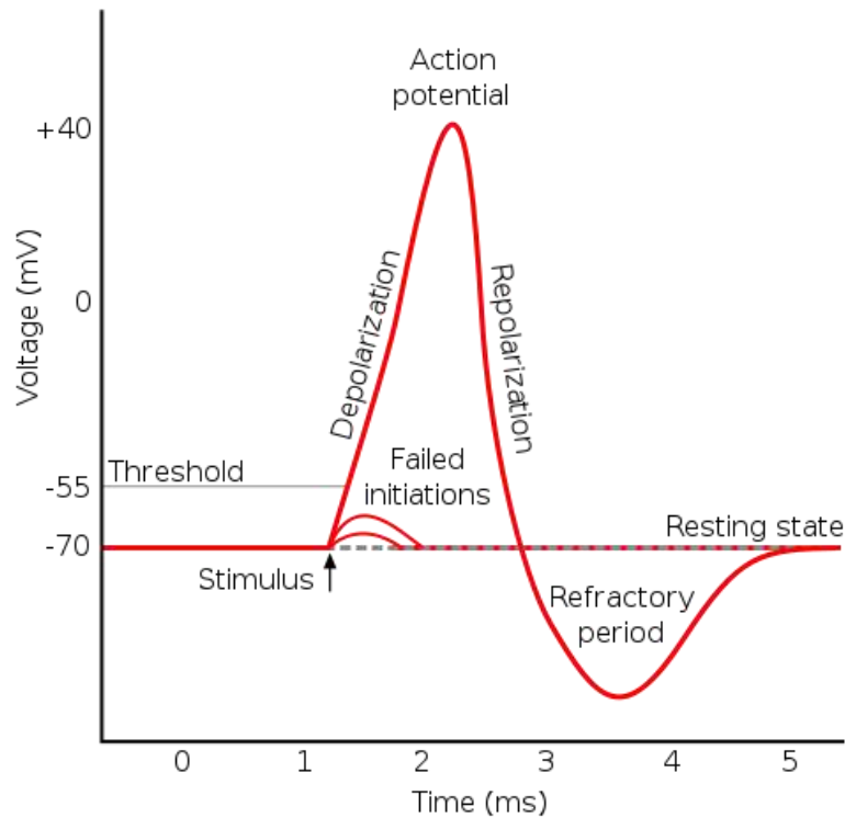
Figure 5: Action potential
