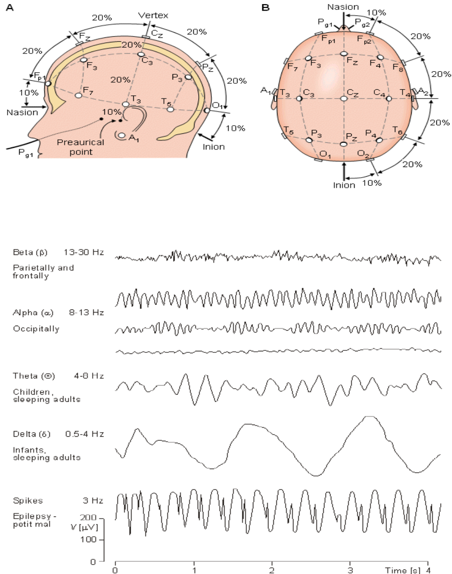
Figure 5: Electroencephalogram
