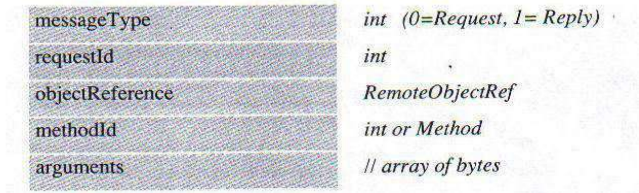
Figure : Request-reply message structure
