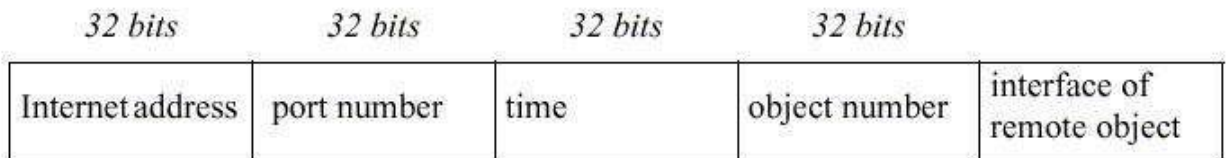
Figure : Representation of a remote object references
