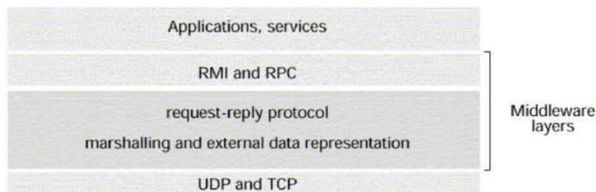
Figure 1. Middleware layers
