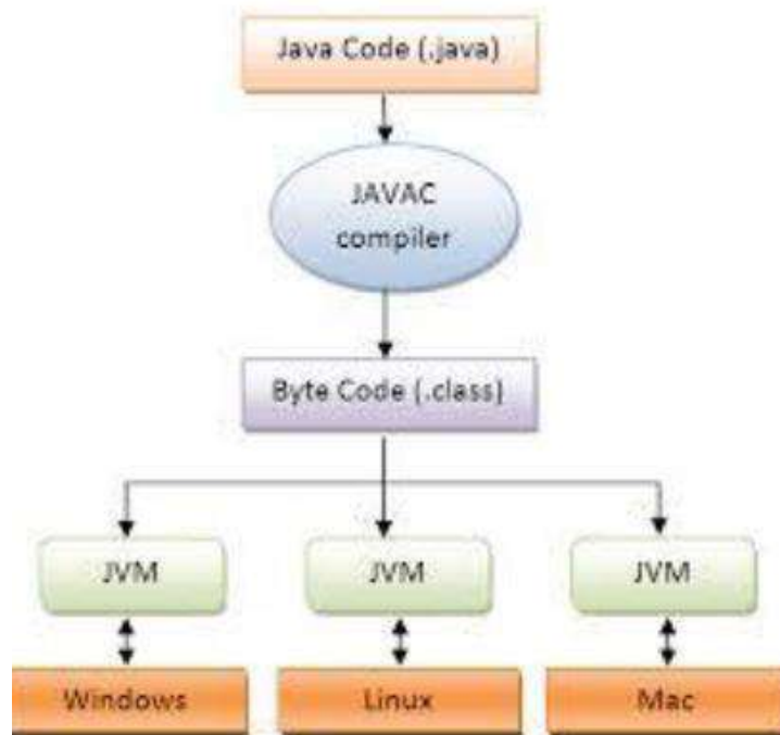
Figure 2 JVM
