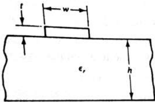
a. Cross-section of Micro strip line
