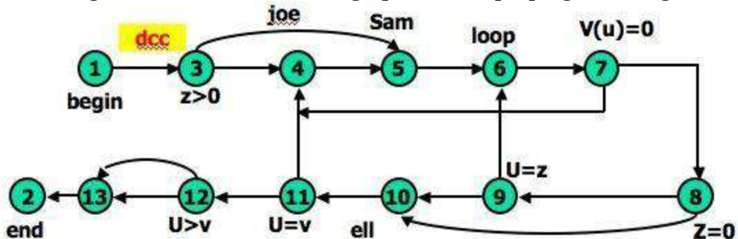
Figure 3.9: Control flow graph annotated for X and Y data flows.
