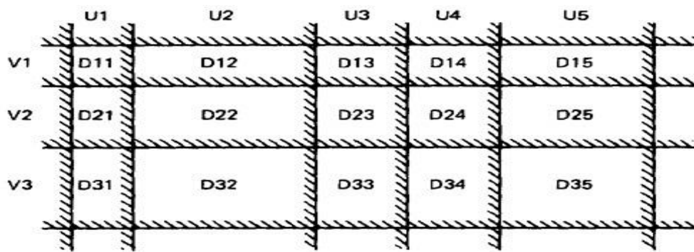
Figure 4.3: Nice Two-Dimensional Domains.
