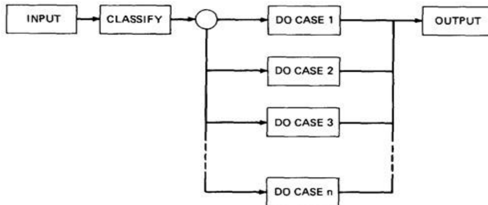
Figure 4.1: Schematic Representation of Domain Testing.
