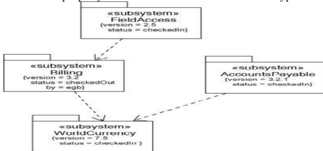
Fig:Modeling New Properties
