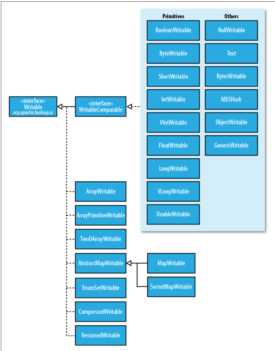
Figure 4-1. Writable class hierarchy
