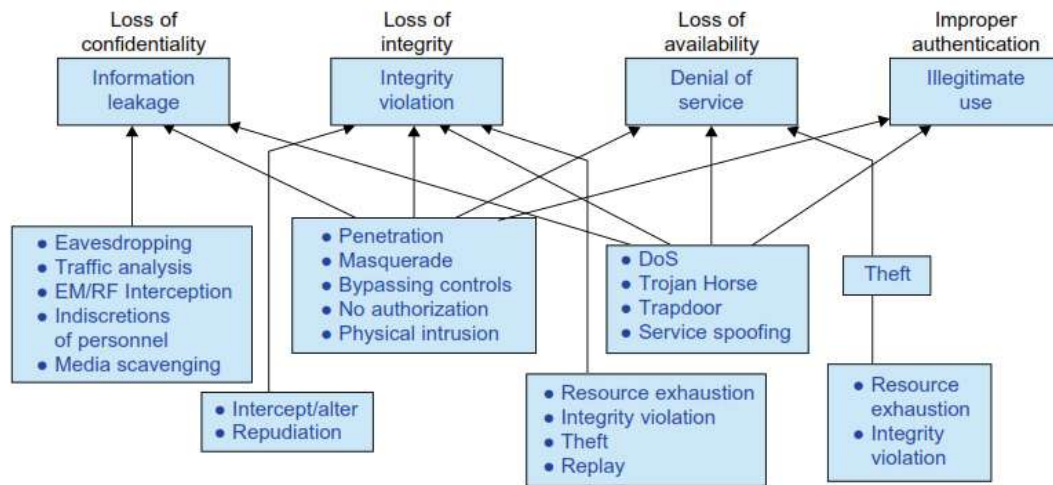
FIGURE 1.25: Various system attacks and network threats to the cyberspace, resulting 4 types of losses.
