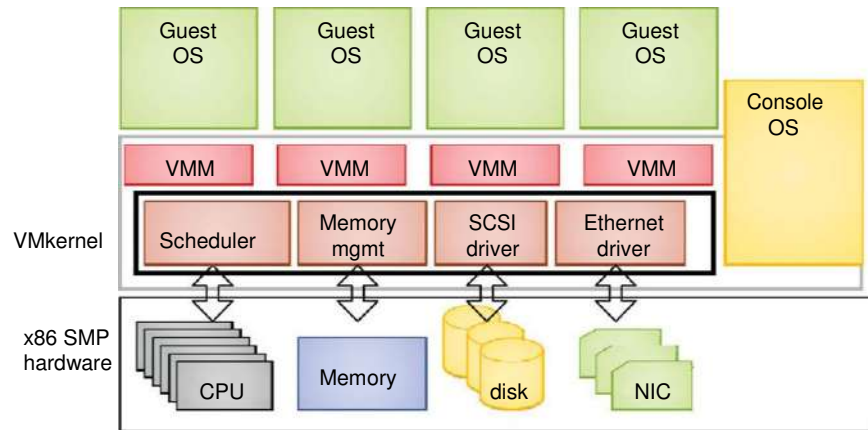
FIGURE 3.9: The VMware ESX server architecture using para-virtualization.
