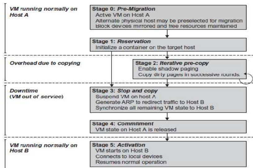
FIGURE 3.20 Live migration process of a VM from one host to another.
