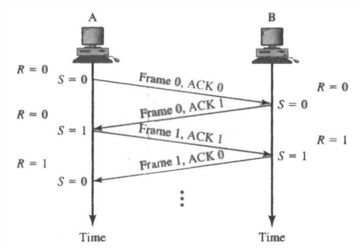
Figure 5: Bidirectional Transmission, Piggybacking
