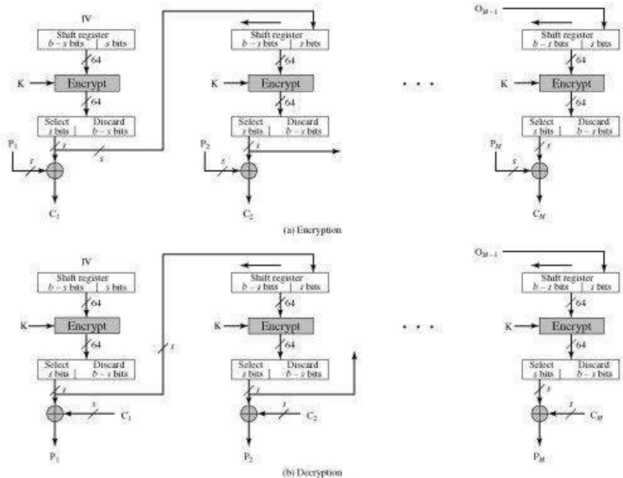
Figure. s-bit Output Feedback (OFB) Mode
