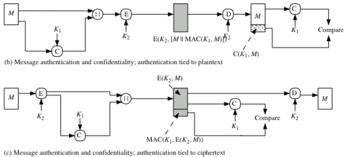
Figure: Basic Uses of Message Authentication Code(MAC)
