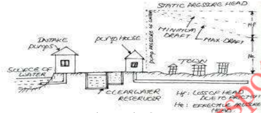
Fig Pumping System
