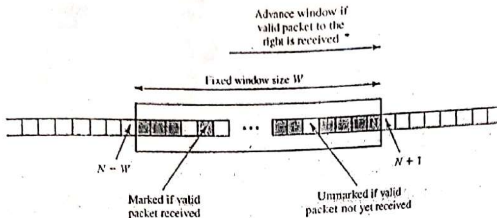
Figure. Antireplay Mechanism
