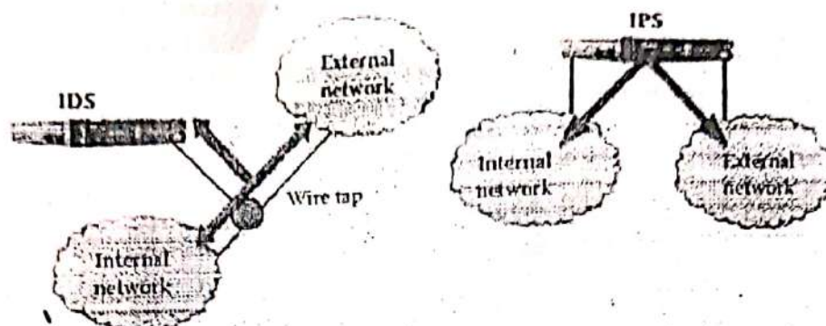
FIGURE 19.2 An illustration of out-of-band IDS vs. in-band IPS.
